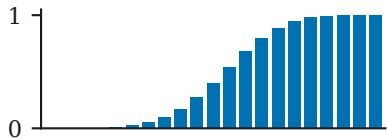
N=20, \varsigma=0.2
