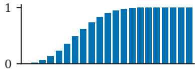
N=20, \varsigma=0.1
