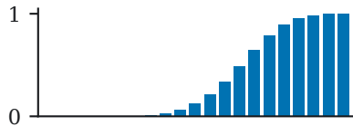
N=20, \varsigma=0.3
